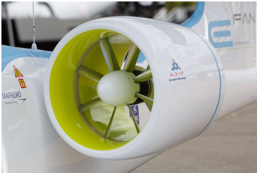
The Airbus E-Fan project used two ducted fan modules. (Credit: Airbus)
